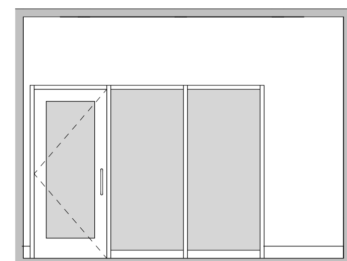
7 STUDY READING ROOM 1/4" = 1'-0"
