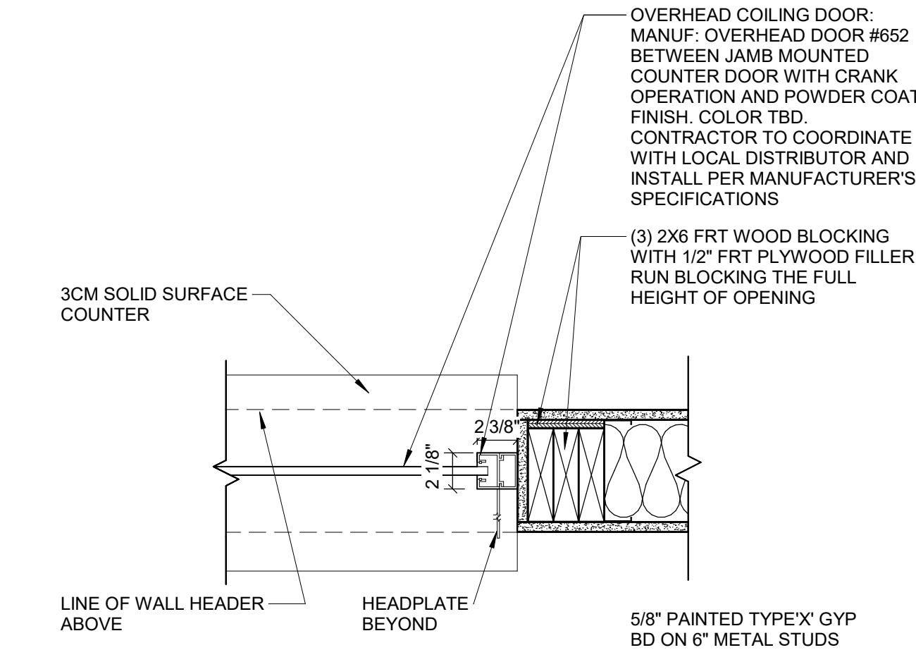
DETAIL JAMB - INTERIOR COILING DOOR AT CONCESSION ② 1 1/2" = 1'-0"
