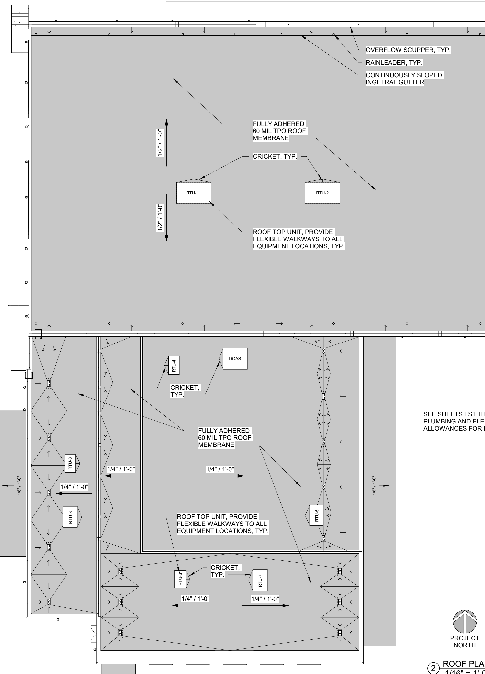
2 ROOF PLAN 1/16" = 1'-0"
