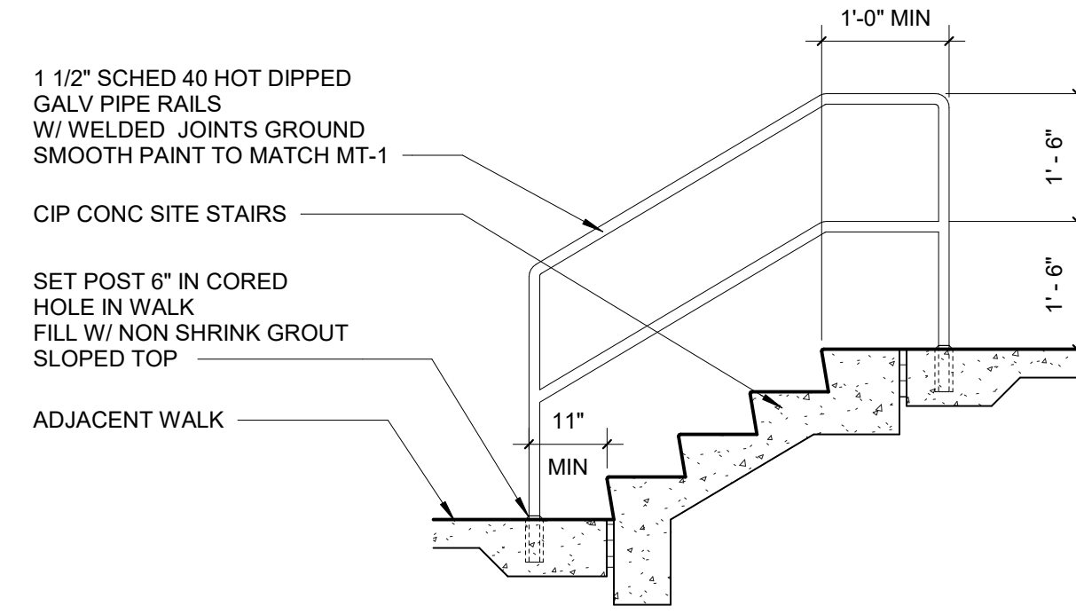
④ SITE SECTION - TYPICAL CONCRETE STAIR 1/2" = 1'-0"
