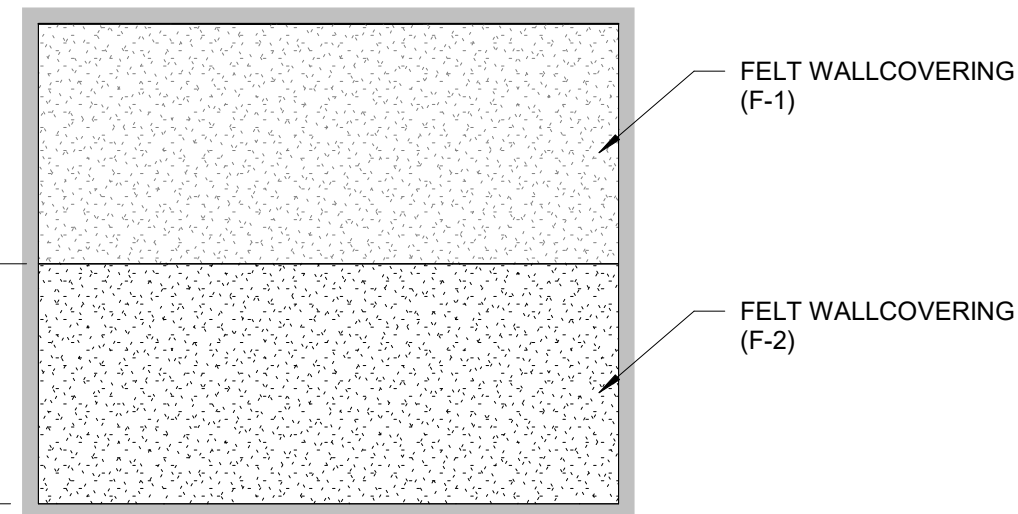
3 RECORDING STUDIO 1/4" = 1'-0"
