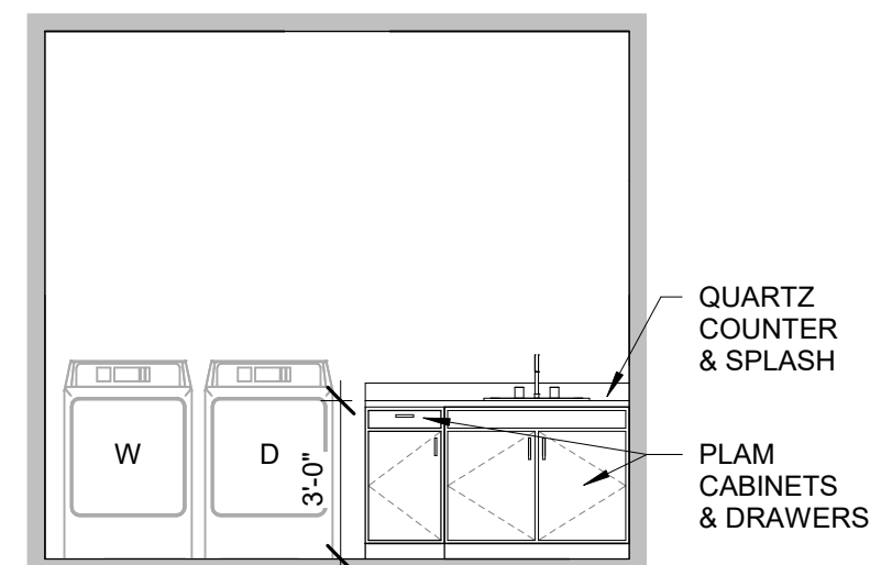
12 LAUNDRY 1/4" = 1'-0"
