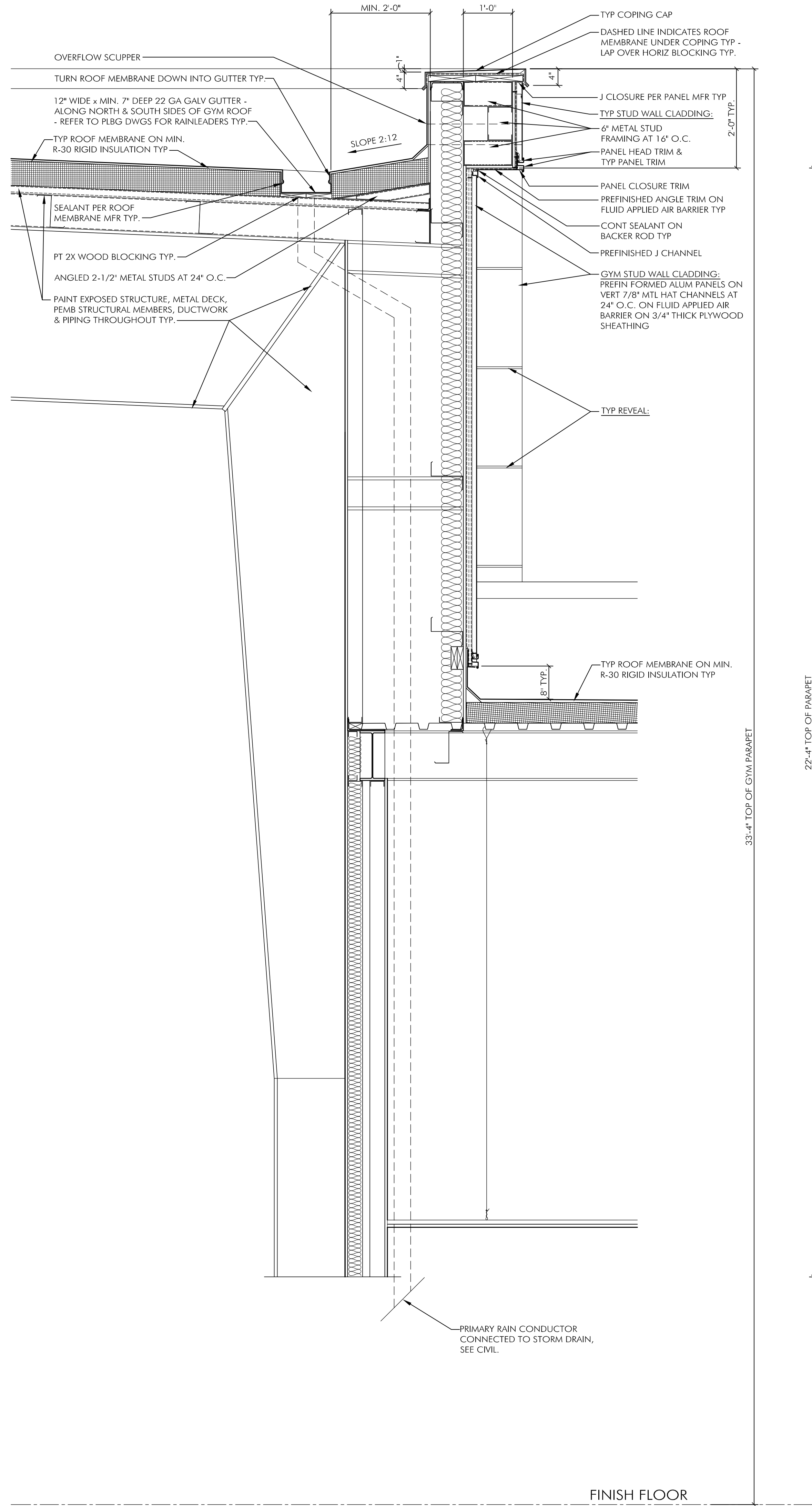
2 WALL SECTION AT INTERMEDIATE ROOF TRANSITION 3/4\" = 1'-0"
