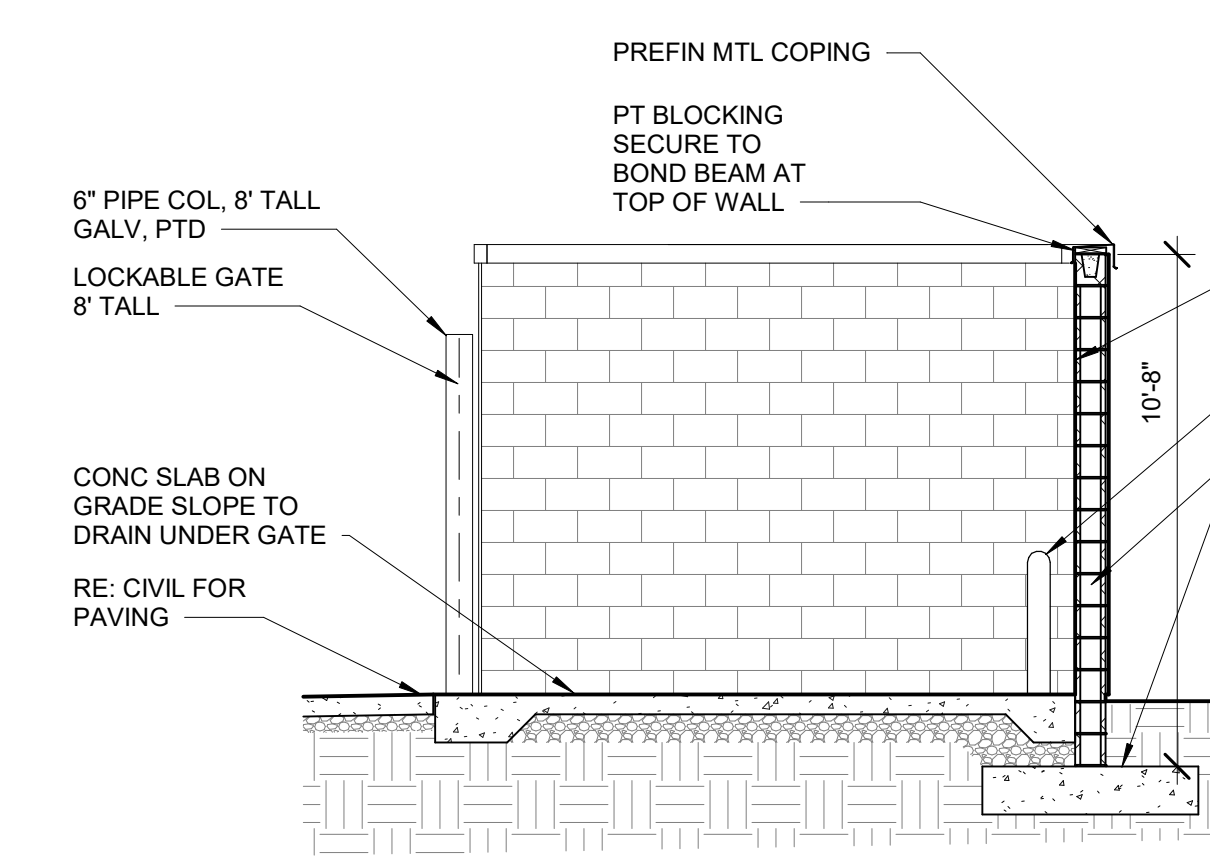
③ SITE SECTION - REFUSE ENCLOSURE 1/4" = 1'-0"
