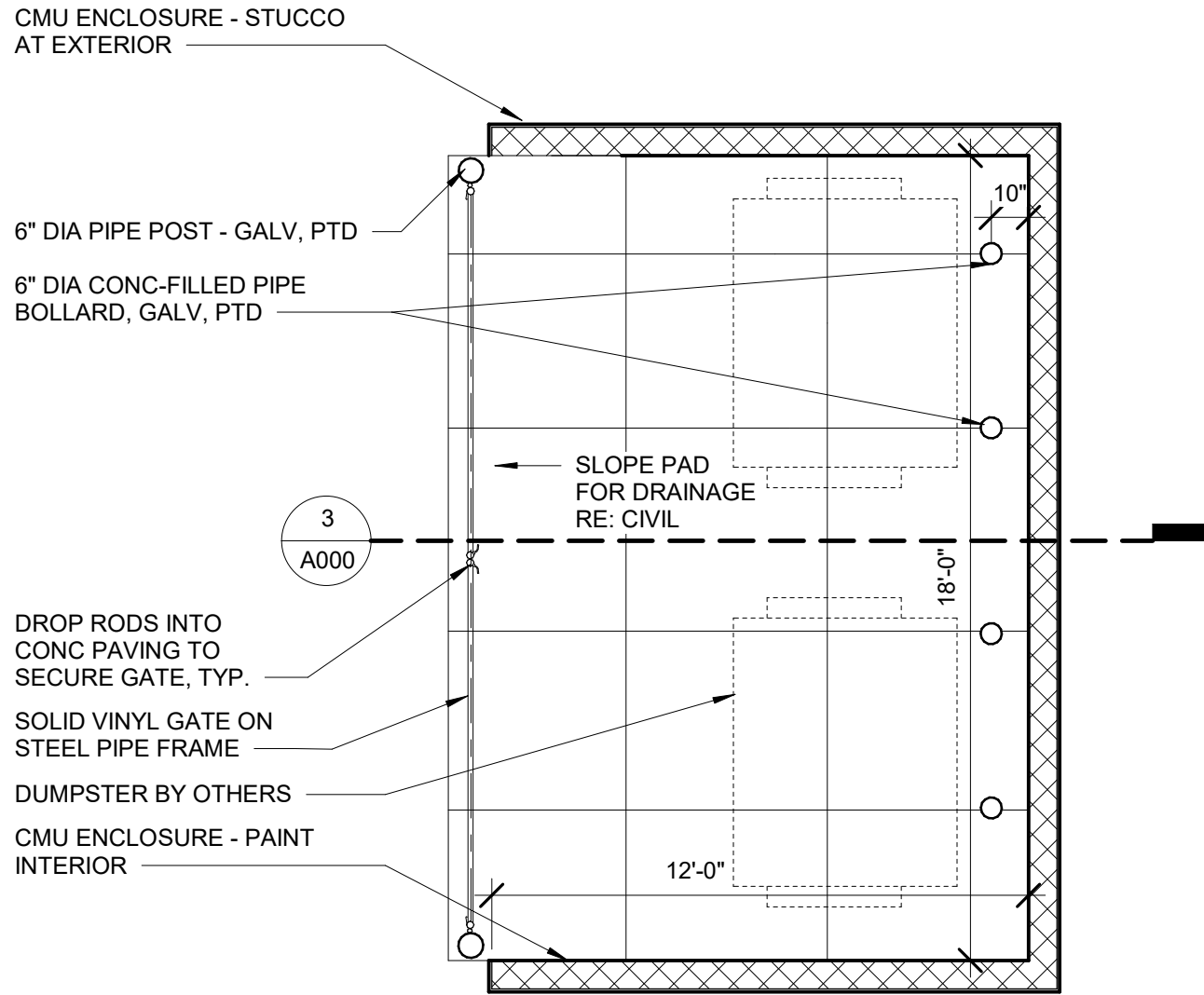
② SITE DETAIL - REFUSE ENCLOSURE 1/4" = 1'-0"
