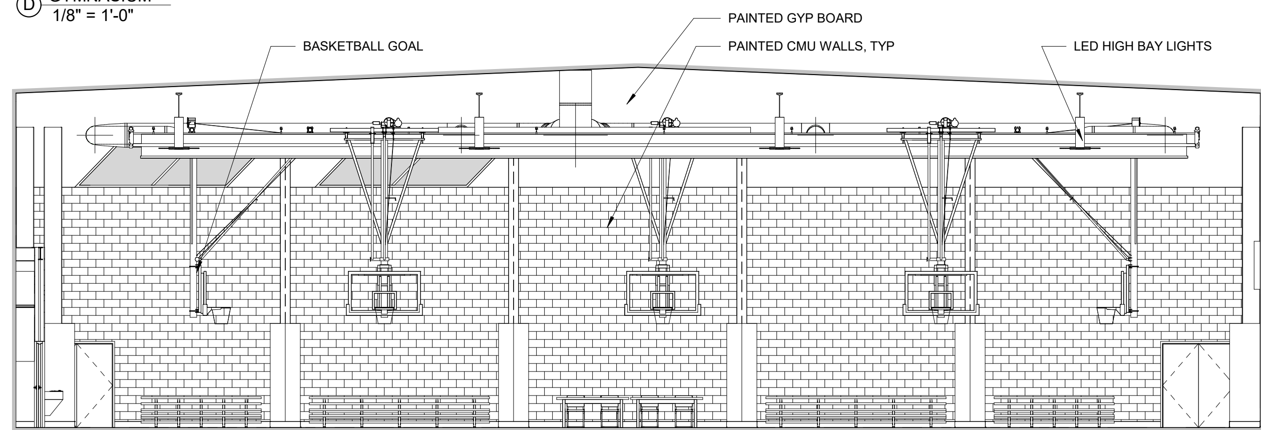
ⓑ GYMNASIUM 1/8" = 1'-0"
