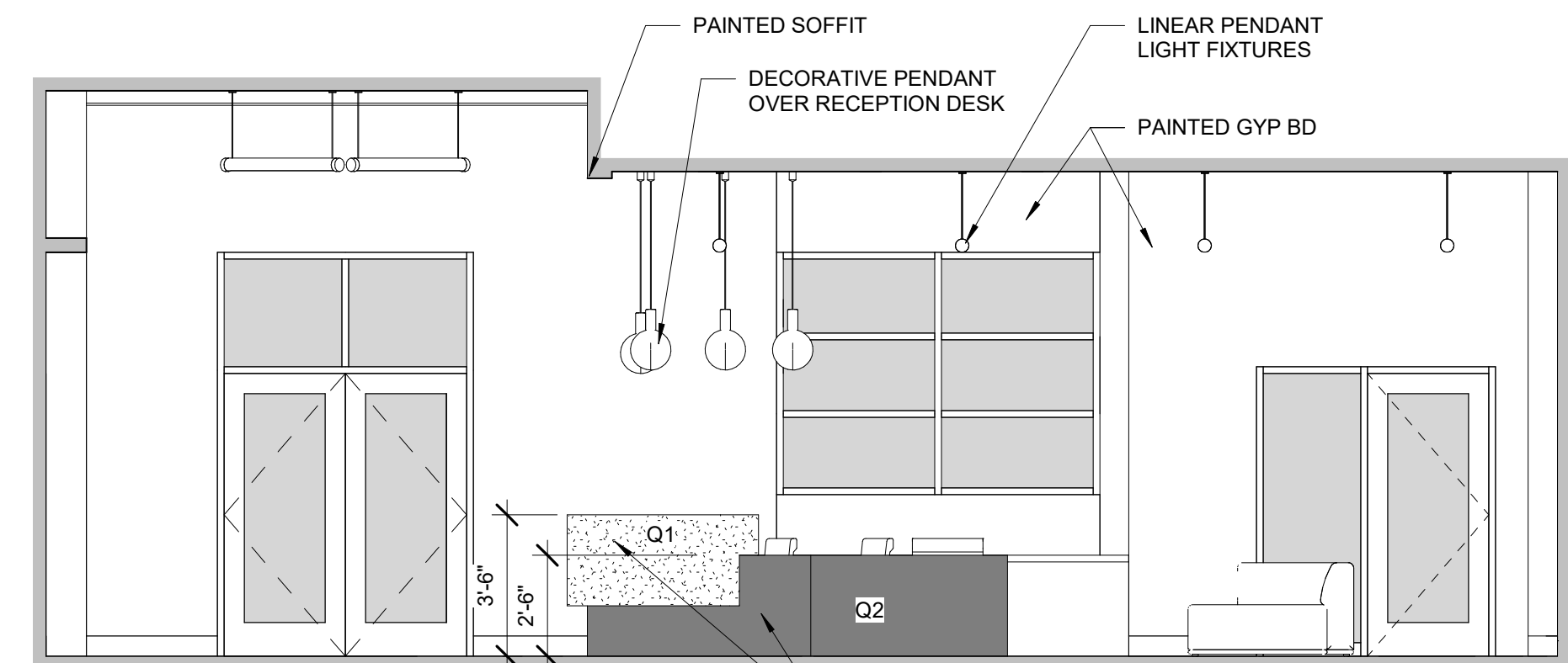
3 RECEPTION 101 1/4" = 1'-0"
