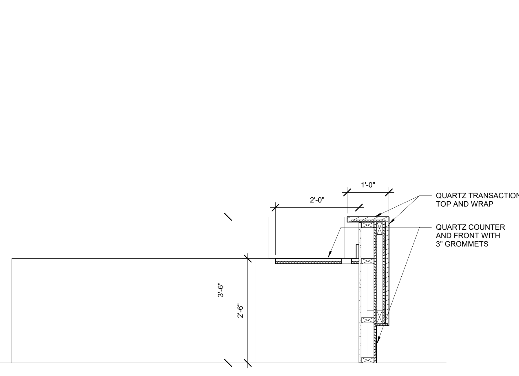
18 RECEPTION DESK 3/4" = 1'-0"
