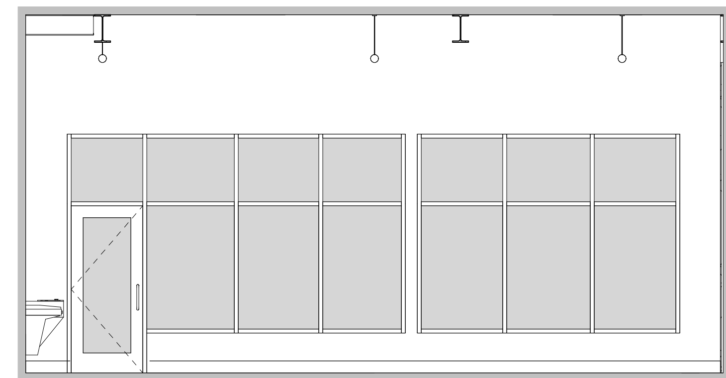
13 FITNESS 1/4" = 1'-0"
