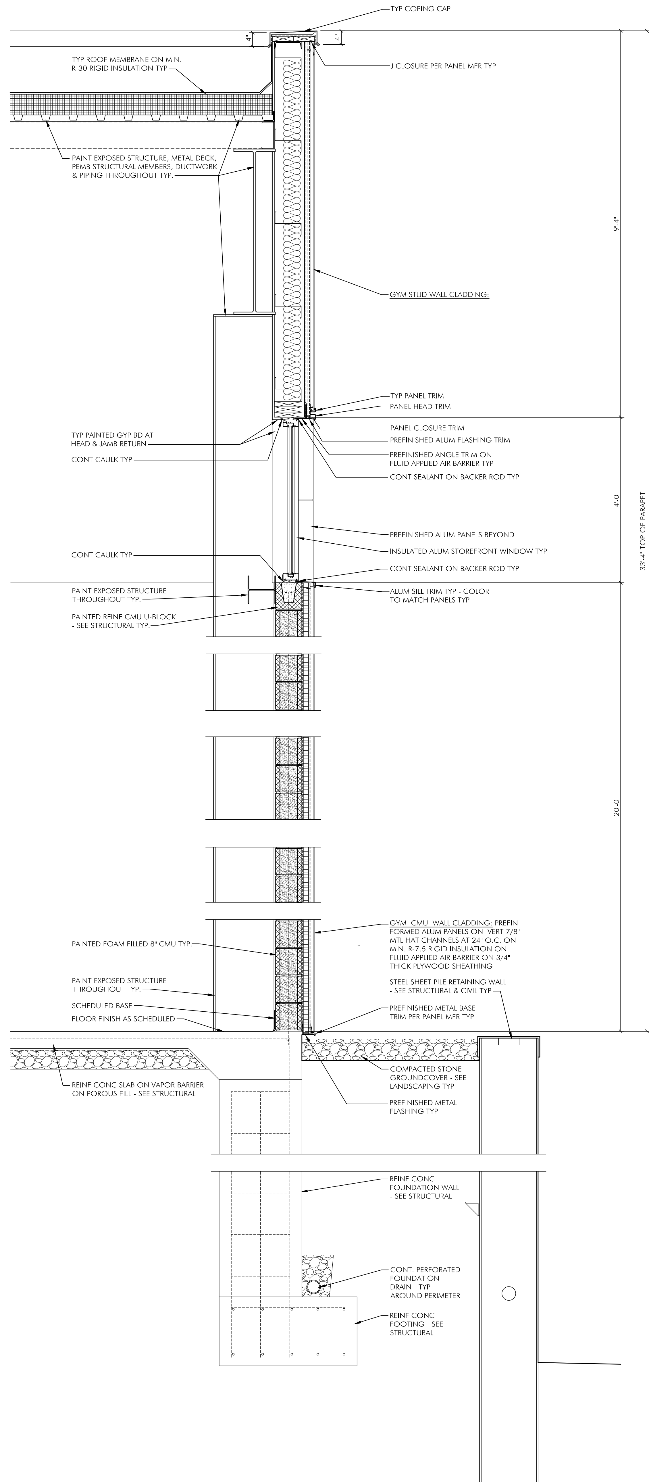
① WALL SECTION AT GYM EAST WALL 3/4" = 1'-0" WEST WALL SIMILAR, OPPOSITE HAND
