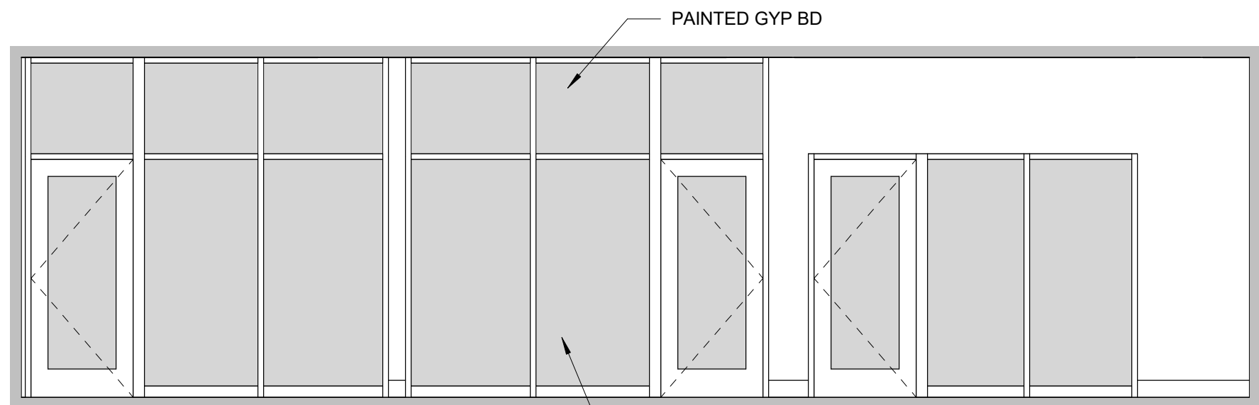
ⓓ CORRIDOR 1/4" = 1'-0"
