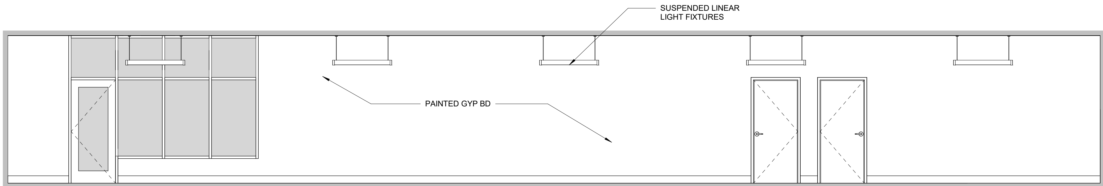
Ⓚ CORRIDOR 1/4" = 1'-0"
