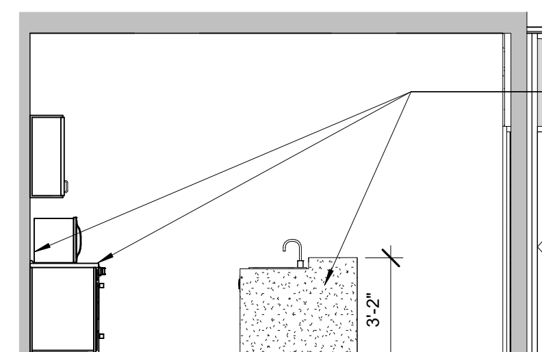
7 TEACHING KITCHEN 1/4" = 1'-0"
