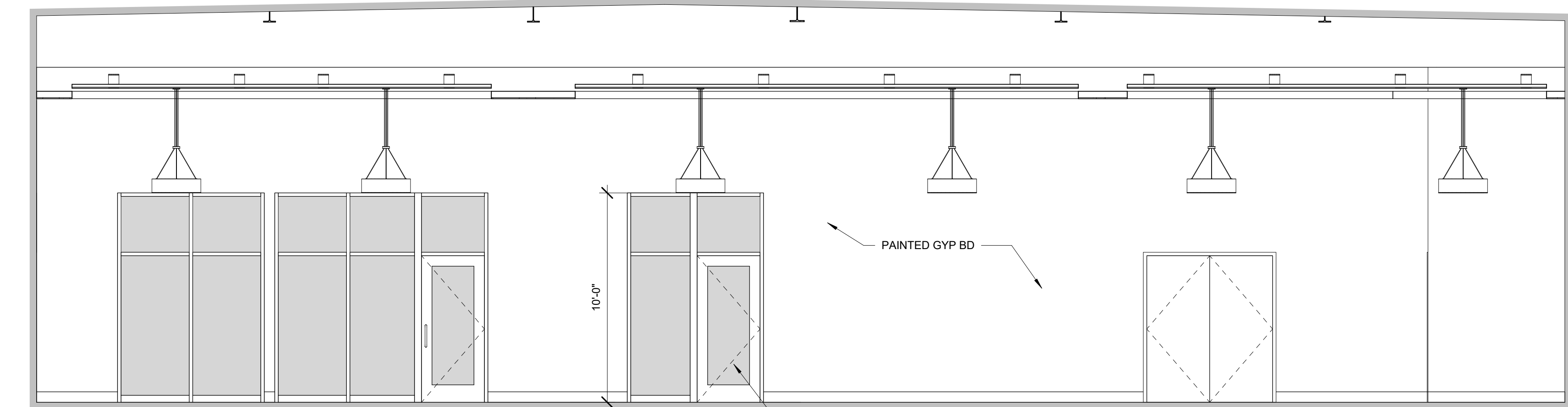
5 MULTI-PURPOSE 1/4" = 1'-0"
