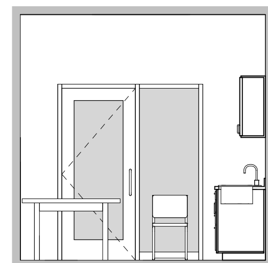
09 FIRST AID 1/4" = 1'-0"
