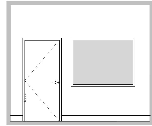
17 ENGINEERING BOOTH 1/4" = 1'-0"
