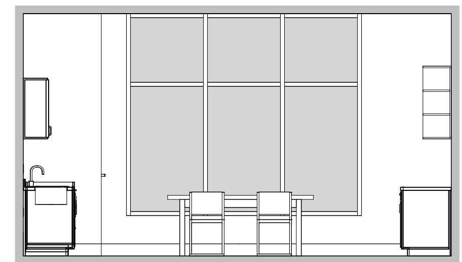
9 ARTS/CRAFTS 1/4" = 1'-0"
