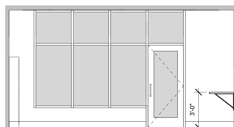
3 ADULT READING 1/4" = 1'-0"
