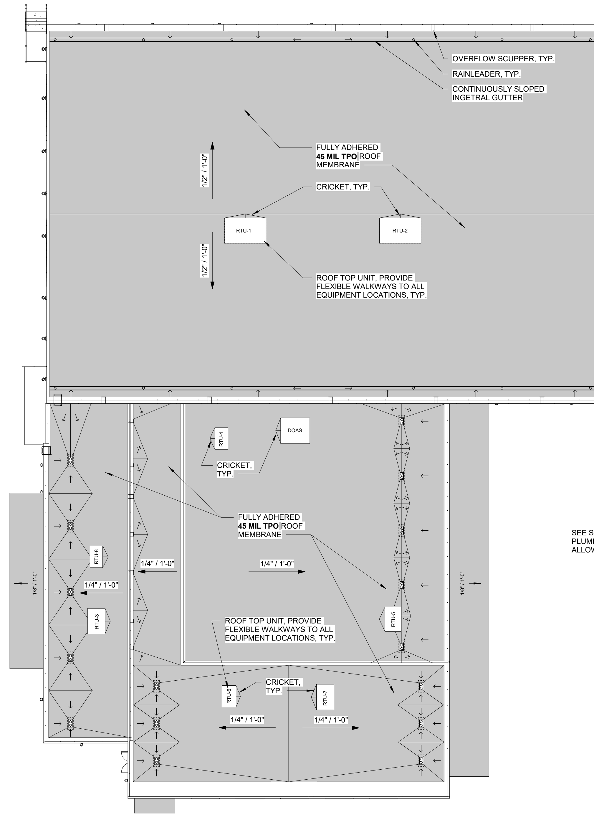
② ROOF PLAN - Alternate 1/16" = 1'-0"
