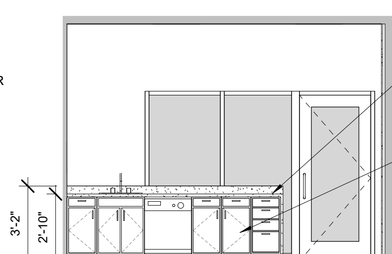
6 TEACHING KITCHEN 1/4" = 1'-0"
