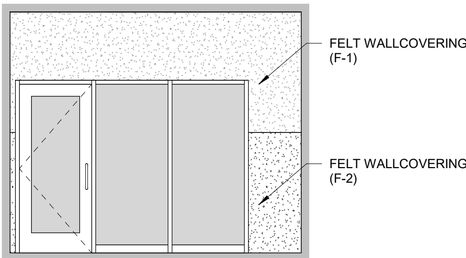
1 RECORDING STUDIO 1/4" = 1'-0"
