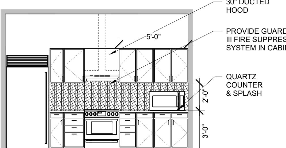
8 TEACHING KITCHEN 1/4" = 1'-0"
