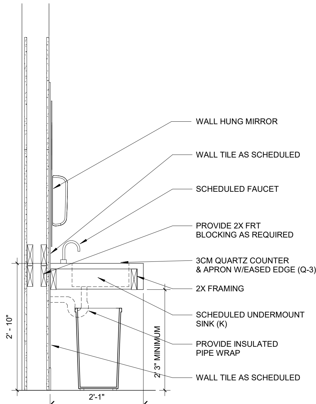
22 LAVATORY SECTION 3/4" = 1'-0"
