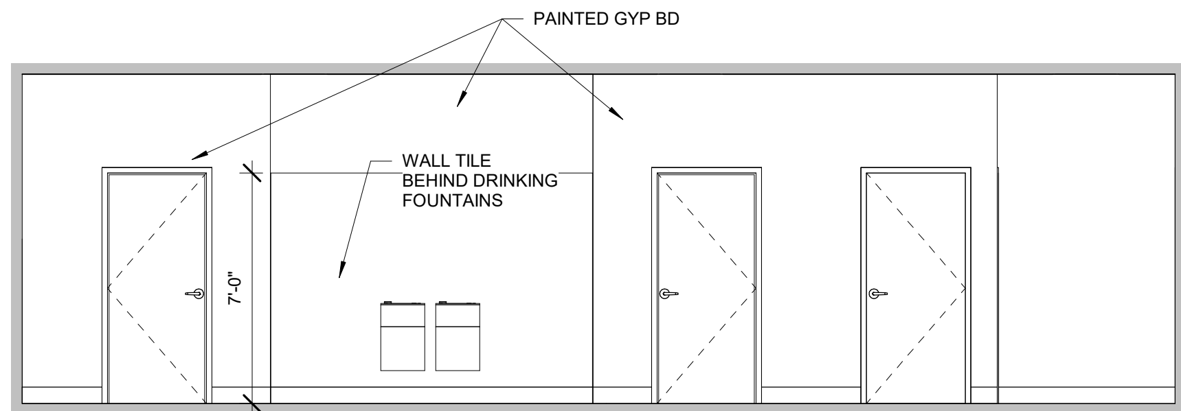
Ⓛ CORRIDOR 1/4" = 1'-0"
