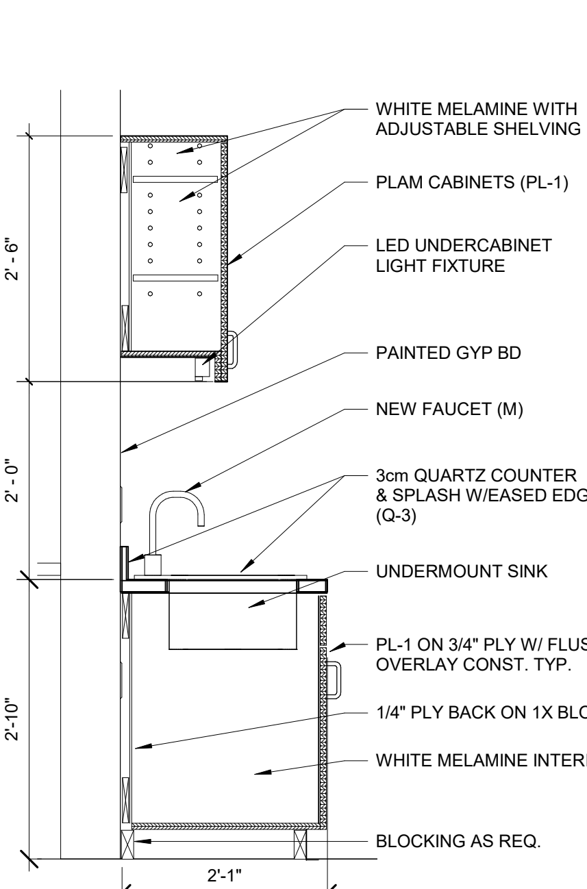
20 MILLWORK SECTION AT SINK 3/4" = 1'-0"
