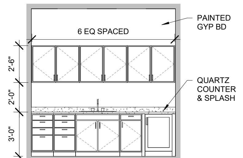
11 FIRST AID 1/4" = 1'-0"
