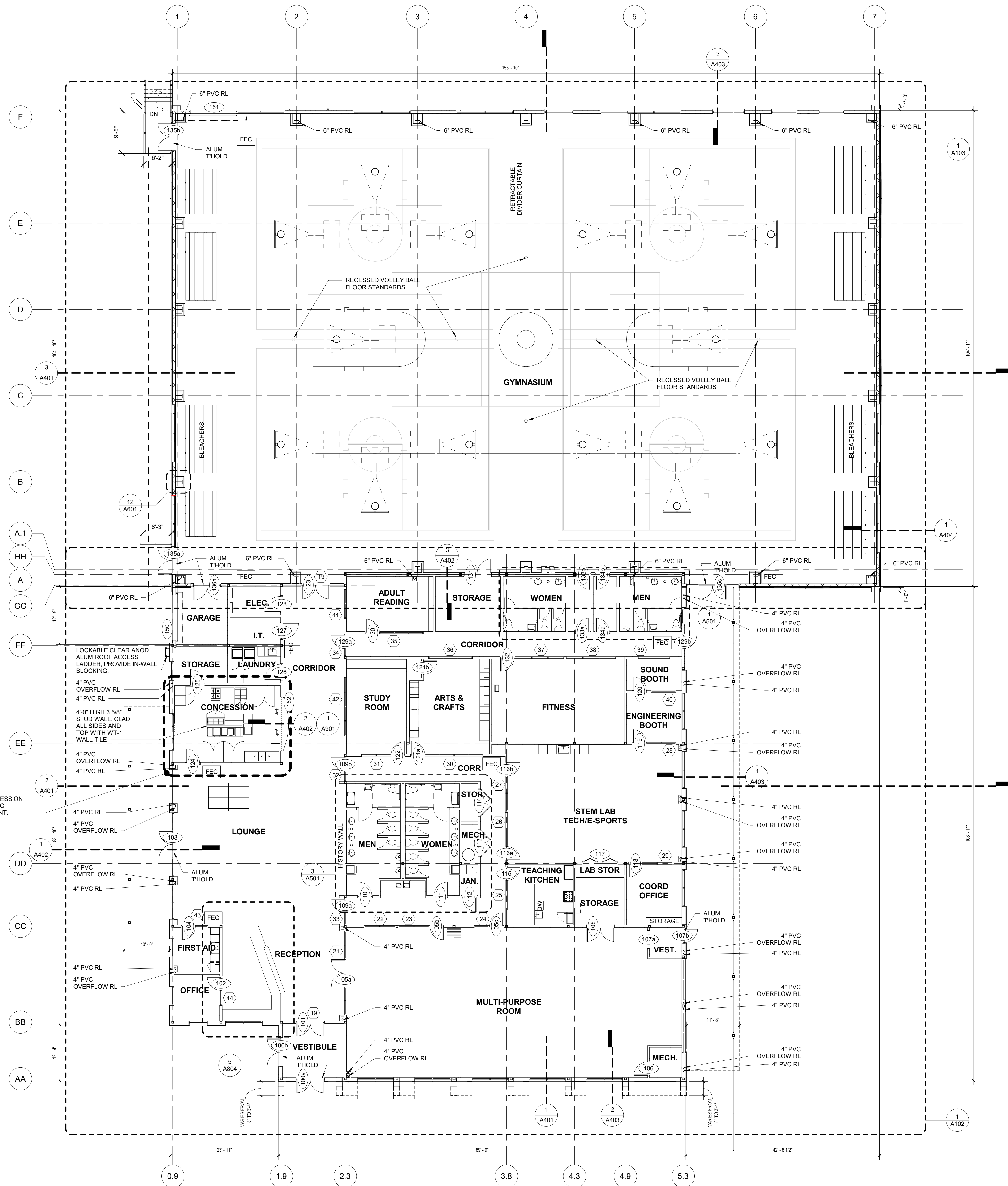
1 FLOOR PLAN - LEVEL 1 1" = 10'-0"
