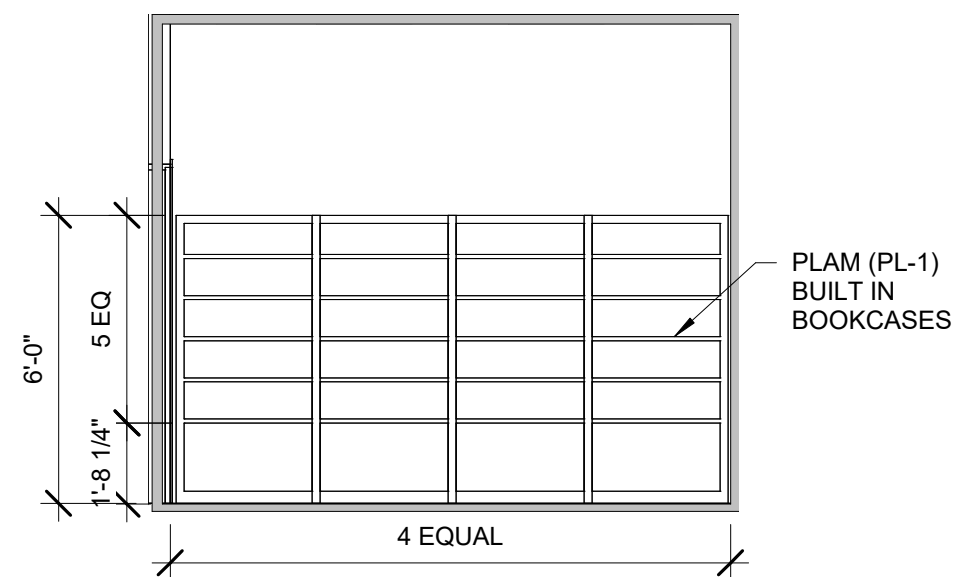
4 ADULT READING 1/4" = 1'-0"
