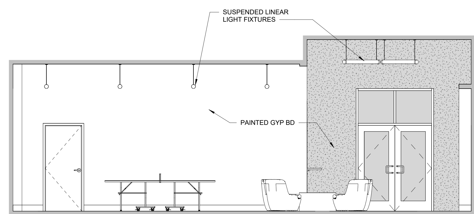
1 RECEPTION 101 1/4" = 1'-0"
