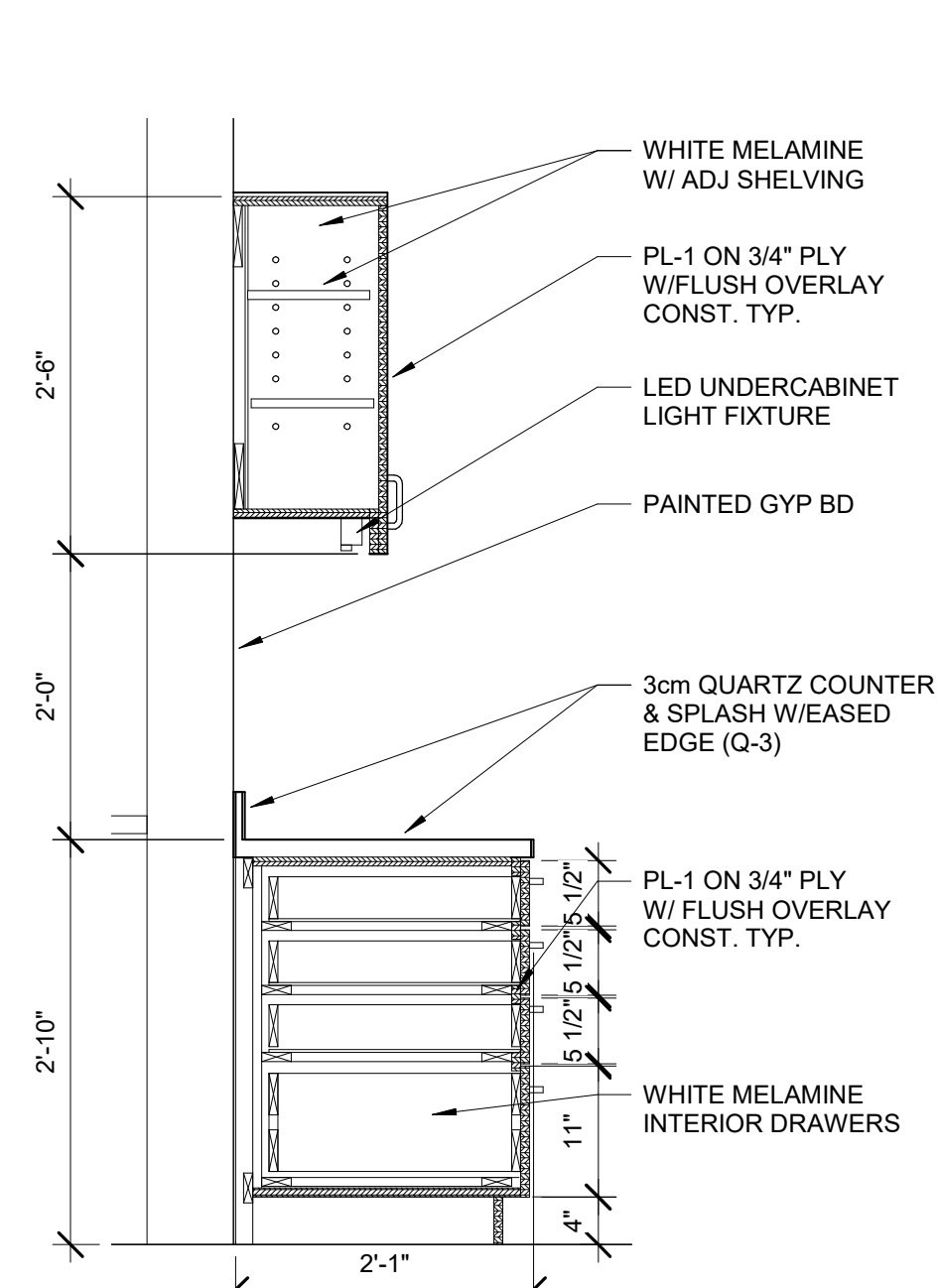
21 FOUR DRAWER MILLWORK SECTION 3/4" = 1'-0"
