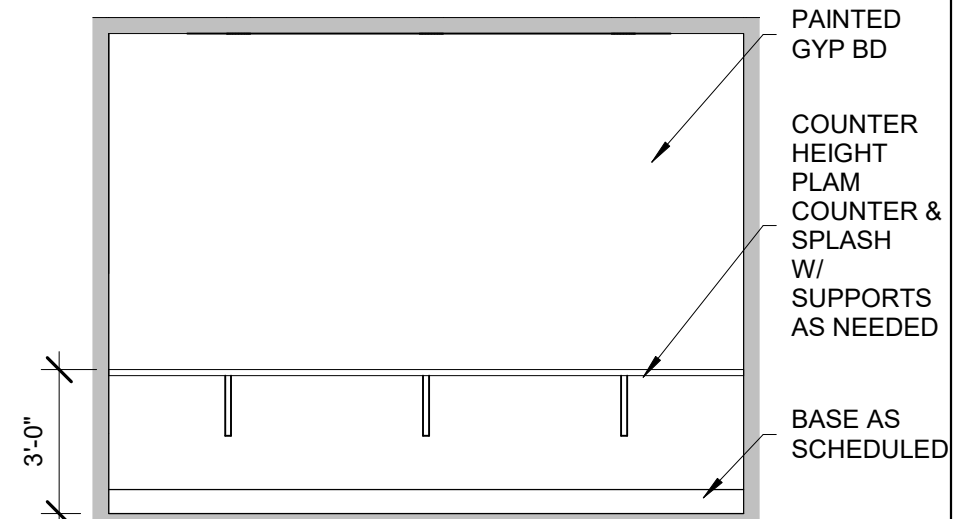
5 STUDY READING ROOM 1/4" = 1'-0"
