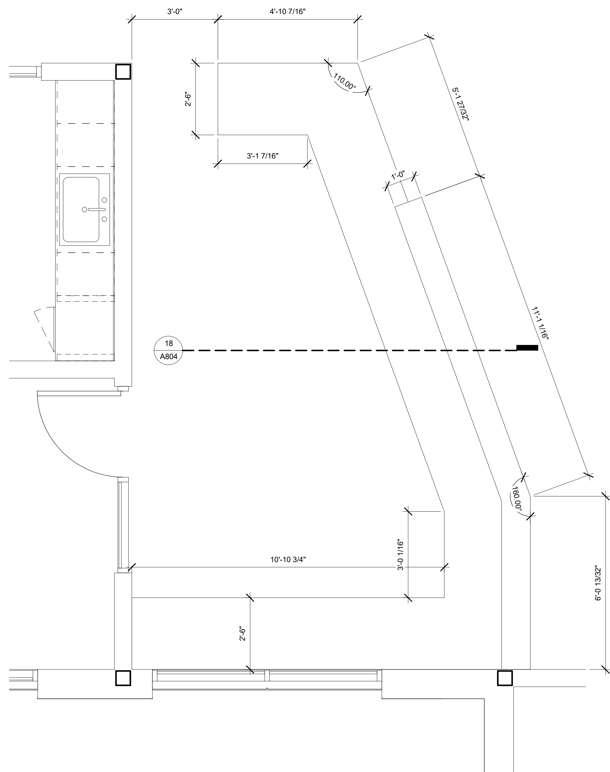
5 RECEPTION DESK ENLARGED PLAN 1/2" = 1'-0"
