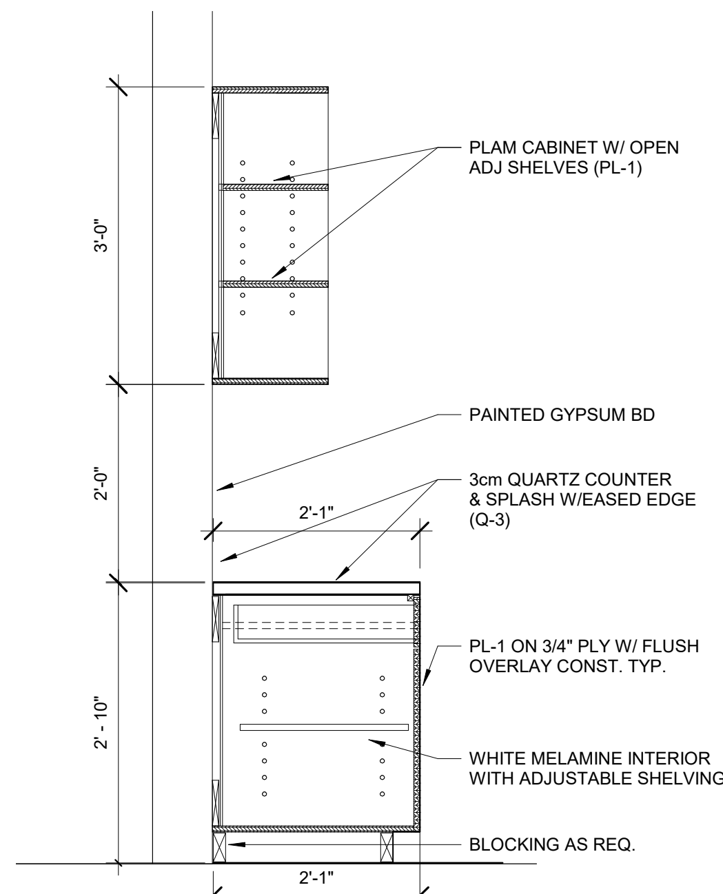
23 MILLWORK SECTION OPEN SHELVES ABOVE 3/4" = 1'-0"
