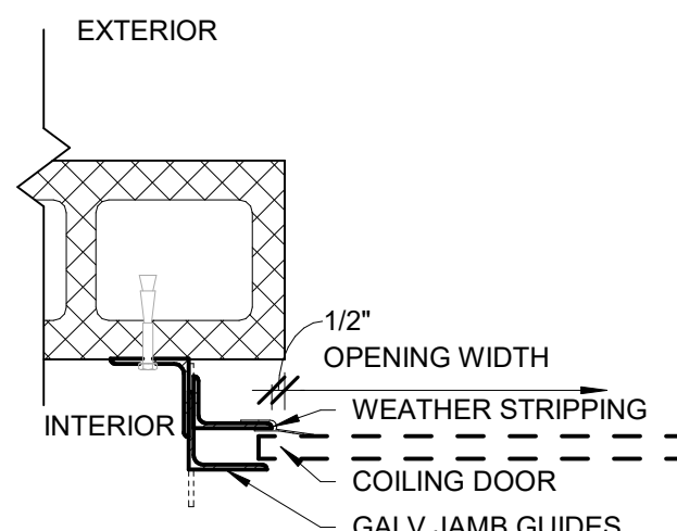
OH COILING DOOR JAMB DETAIL SCALE 1 1/2" = 1'-0"
