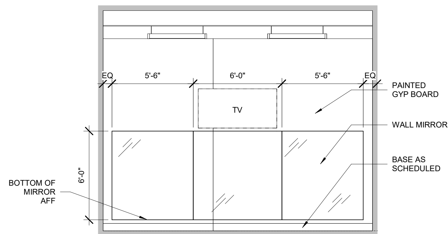
16 FITNESS 1/4" = 1'-0"
