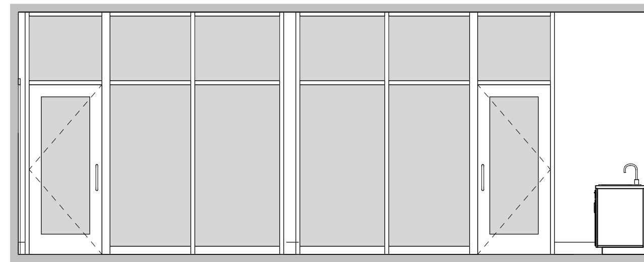
22 STEM LAB 1/4" = 1'-0"
