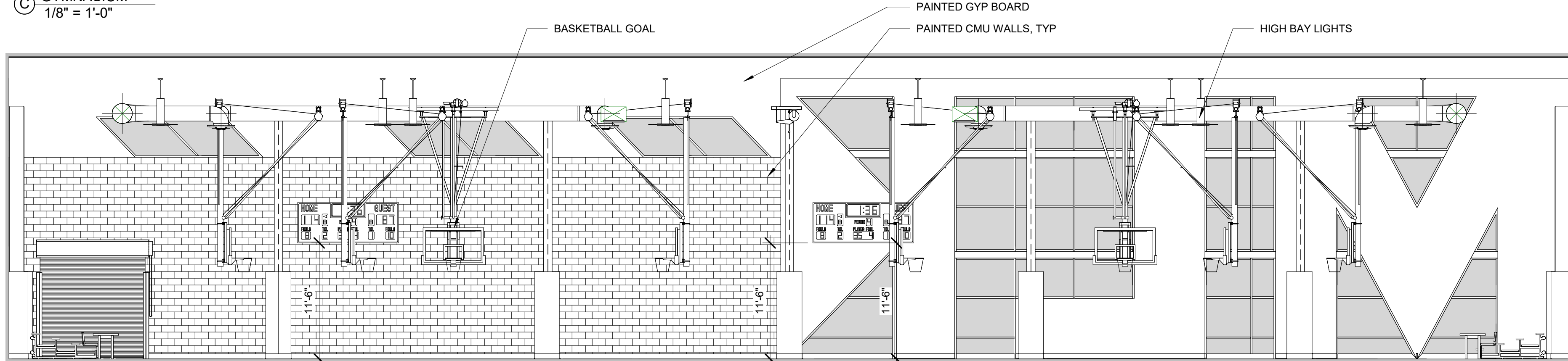
ⓐ GYMNASIUM 1/8" = 1'-0"
