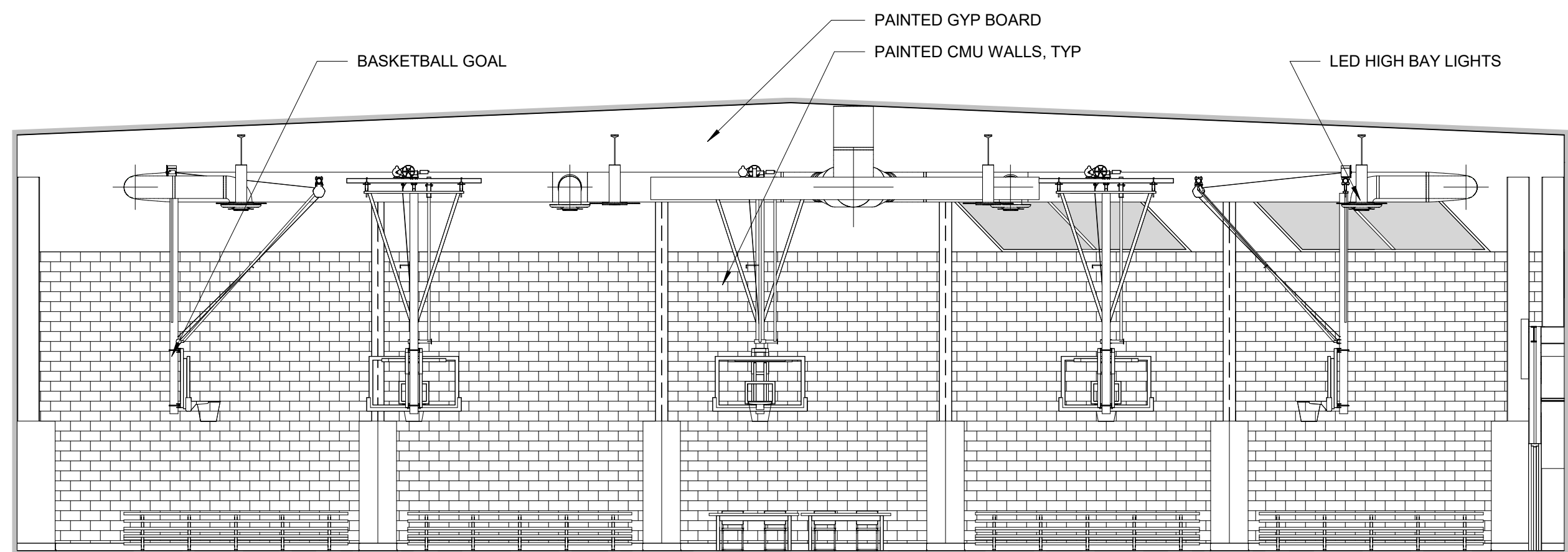
ⓓ GYMNASIUM 1/8" = 1'-0"
