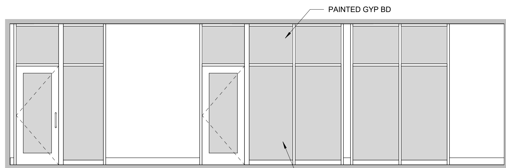
Ⓝ CORRIDOR 1/4" = 1'-0"
