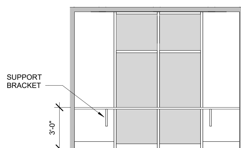
2 ADULT READING 1/4" = 1'-0"
