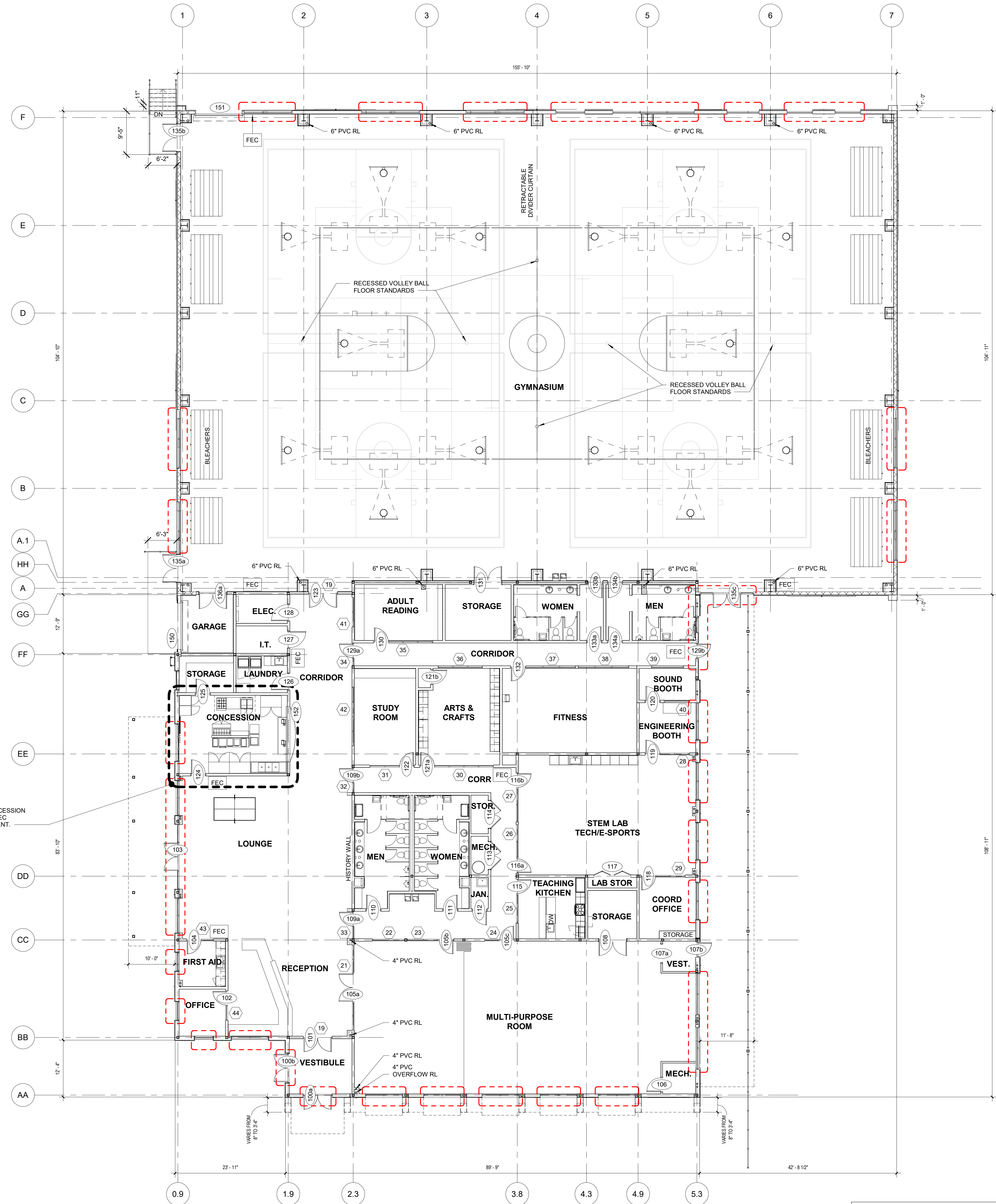
① FLOOR PLAN - LEVEL 1 Alternate 1" = 10'-0"
