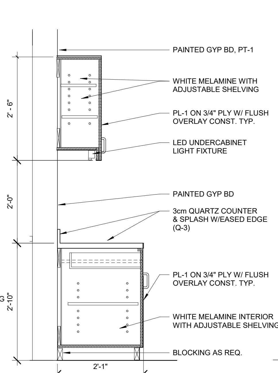
19 MILLWORK SECTION 3/4" = 1'-0"
