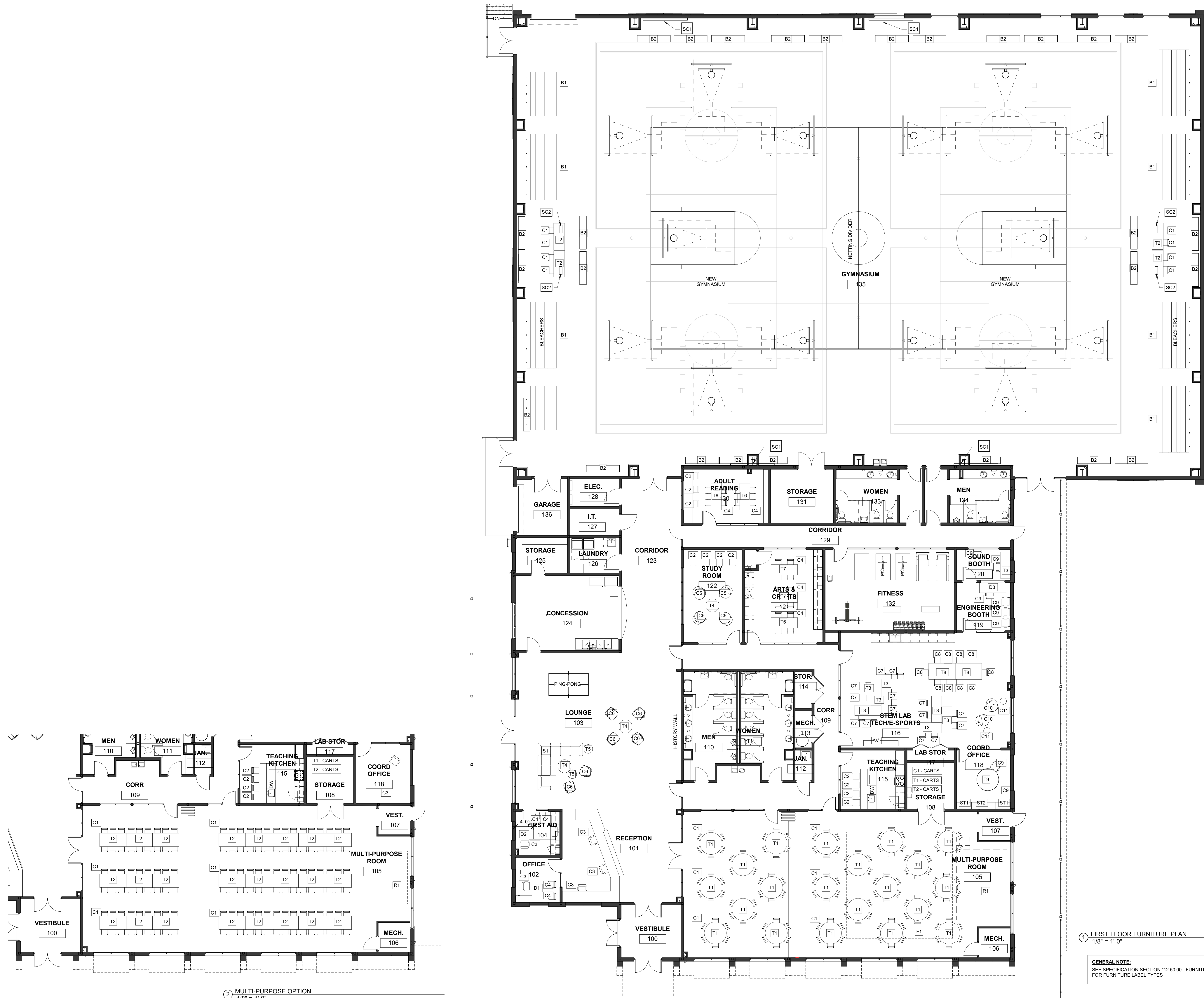
② MULTI-PURPOSE OPTION 1/8" = 1'-0"
