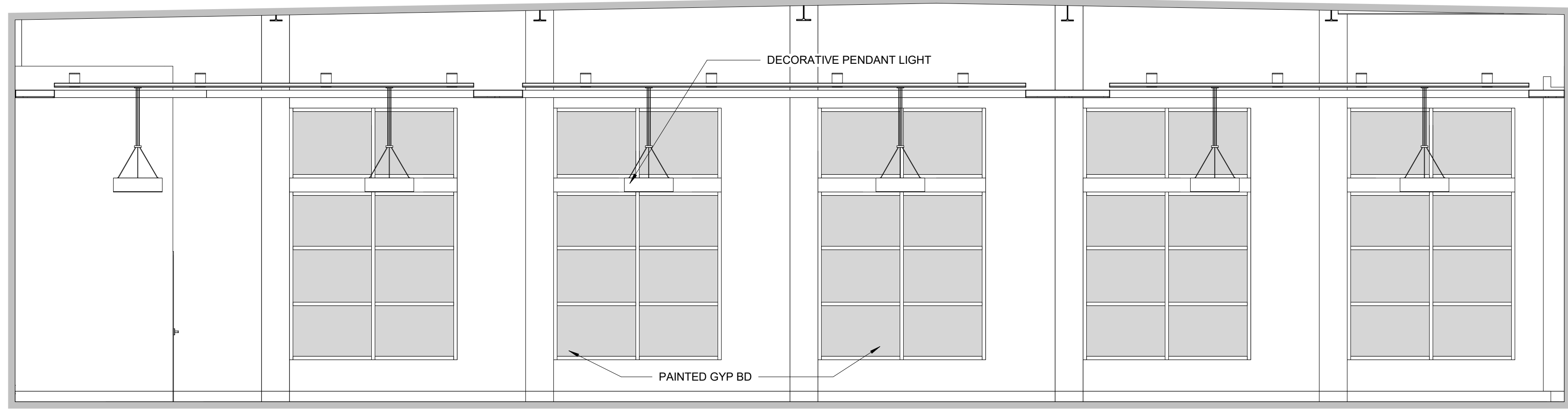
7 MULTI-PURPOSE 1/4" = 1'-0"
