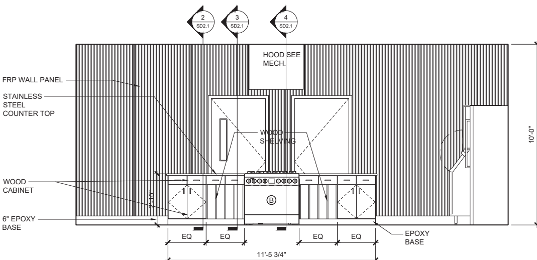
A WARMING KITCHEN 102 ELEVATION SD2.1 SCALE: 3/8" = 1'-0"
