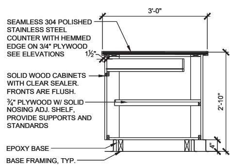
2 CABINET DETAIL SD2.1 SCALE: 3/4" = 1'-0"
