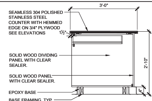
3 CABINET DETAIL SD2.1 SCALE: 3/4" = 1'-0"
