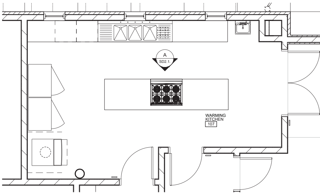
1 WARMING KITCHEN 107 LARGE SCALE PLAN SD2 SCALE: 3/8"=1'-0"
