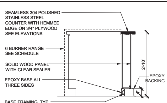
4 CABINET DETAIL SD2.1 SCALE: 3/4" = 1'-0"
