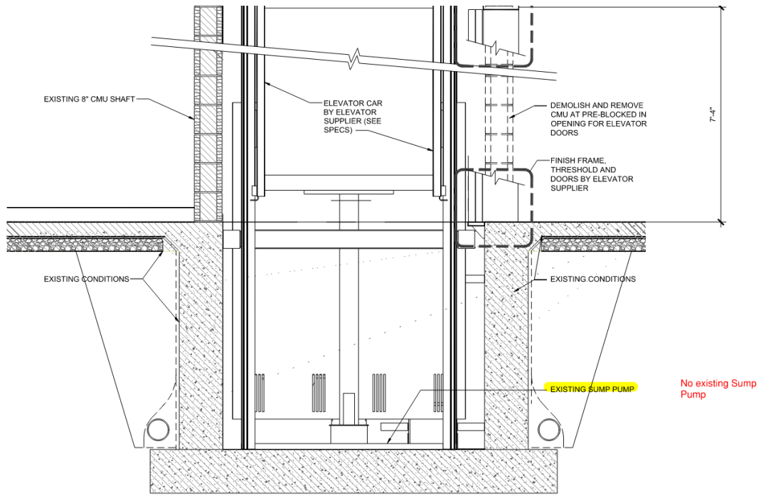
A WALL SECTION SCALE: 3/4"=1'-0"
